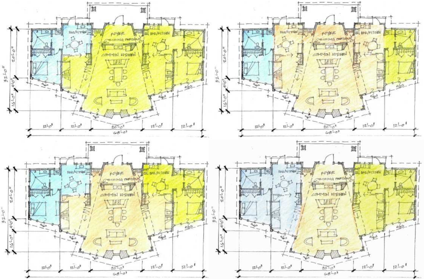
Floor Plan Layout Scenarios
